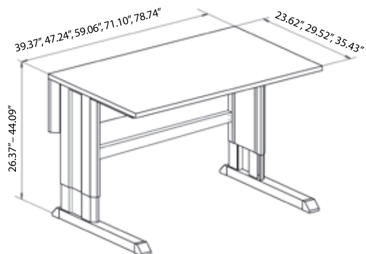
Lab Bench, manual adjustment
