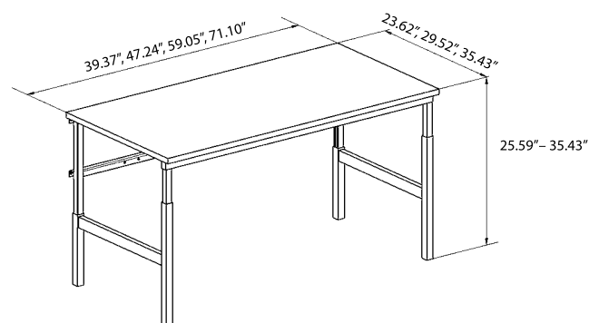
Basic Lab Bench
